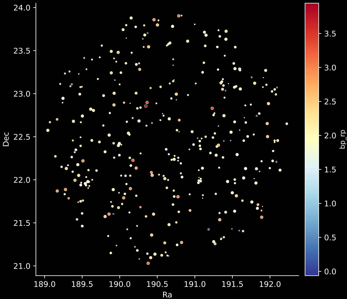
APOGEE DR17 Field: [188+00] Stars: 348
