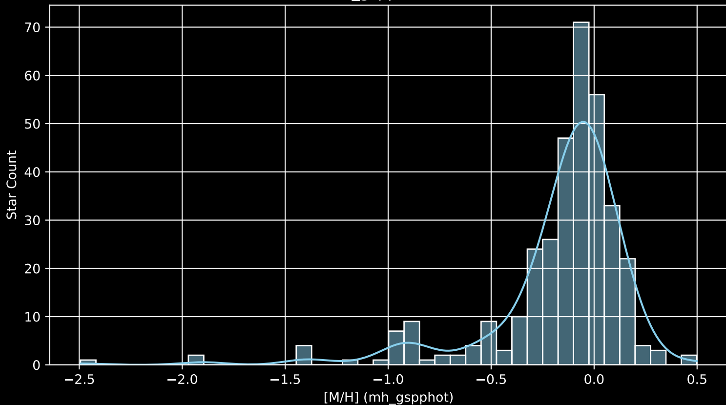
APOGEE DR17 Field: [188+00 [M/H] (mh_gspphot) (n= 344)
