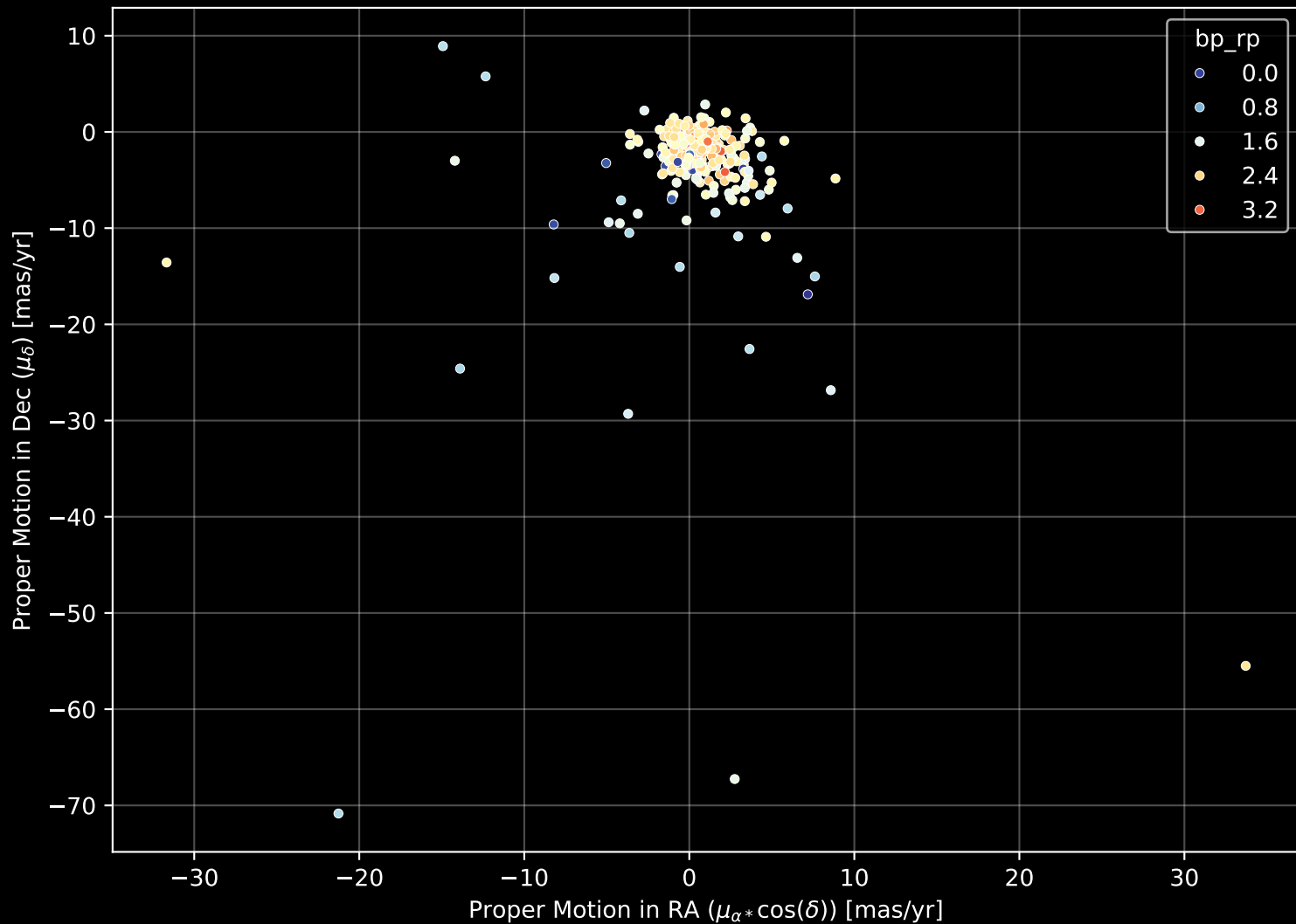
APOGEE DR17 Field: [188+00] Proper Motion Diagram (n= 348)
