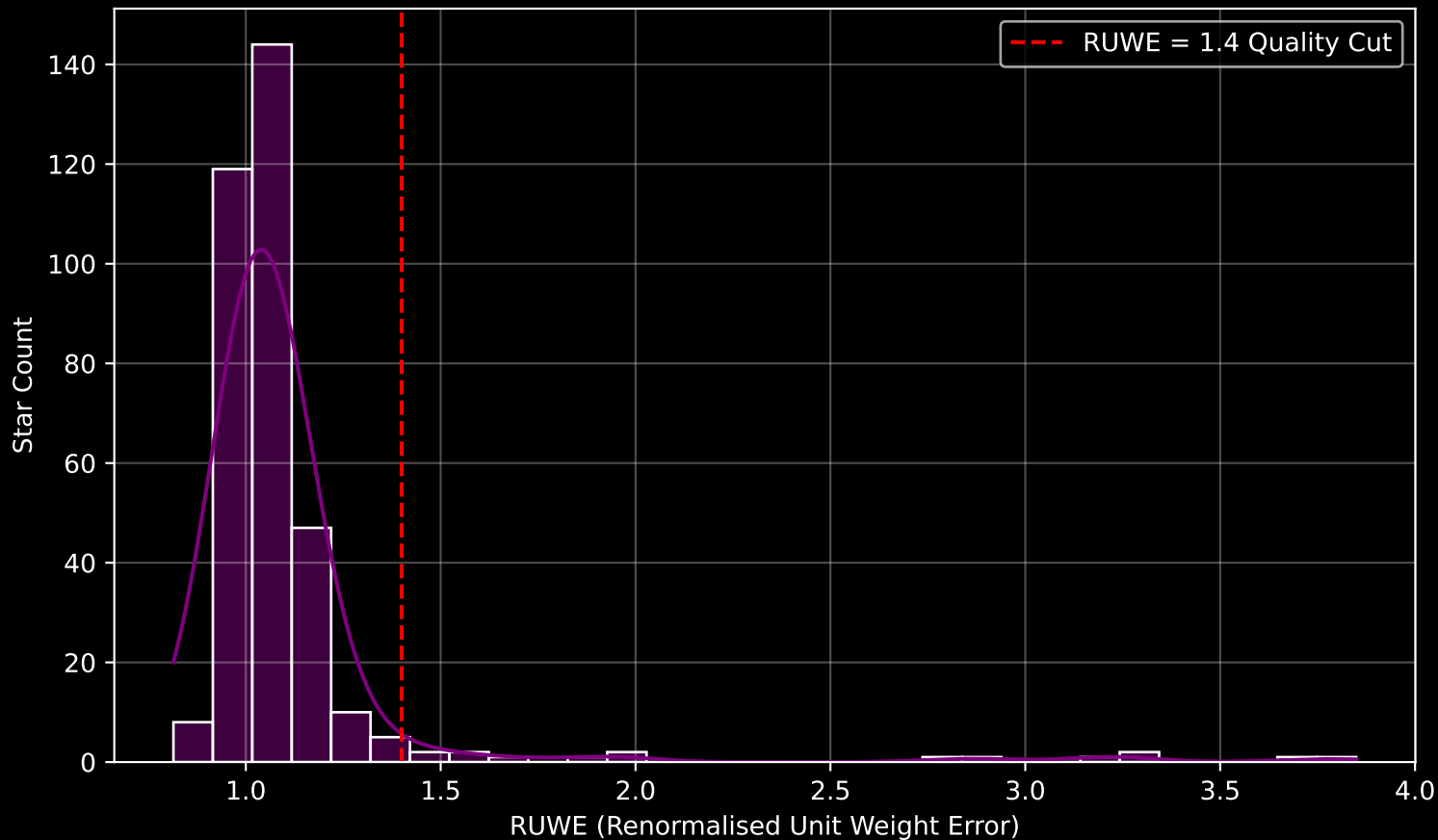
GAPOGEE DR17 Field [188+00] RUWE Distribution (n= 348)
