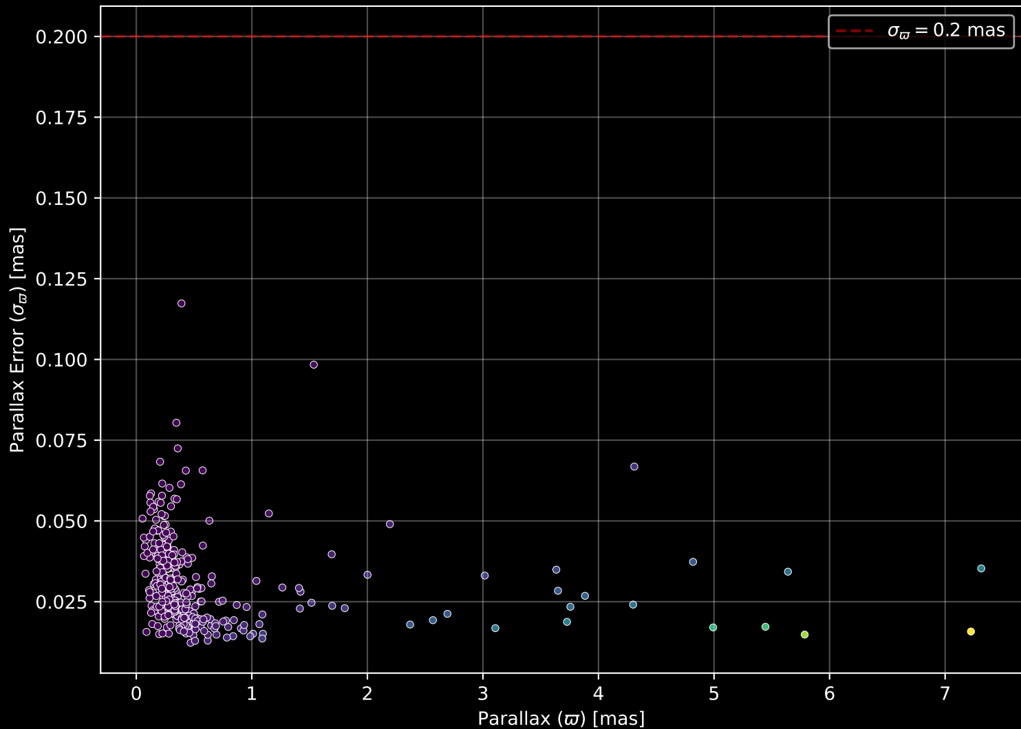
APOGEE DR17 Field: [188+00] Parallax Quality (n= 348)
