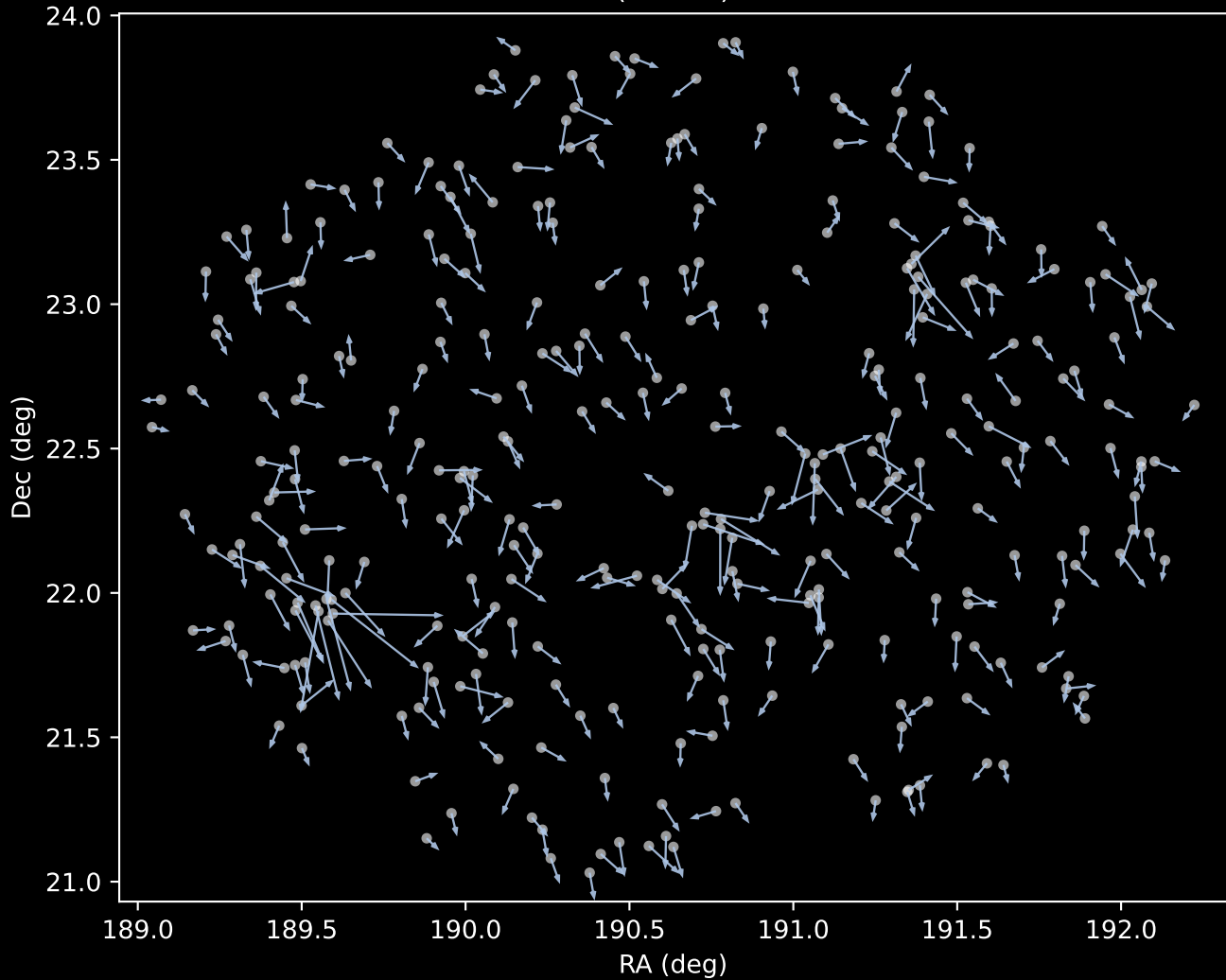
APOGEE DR17 Cluster 1 Proper Motion Vectors (n=320)
