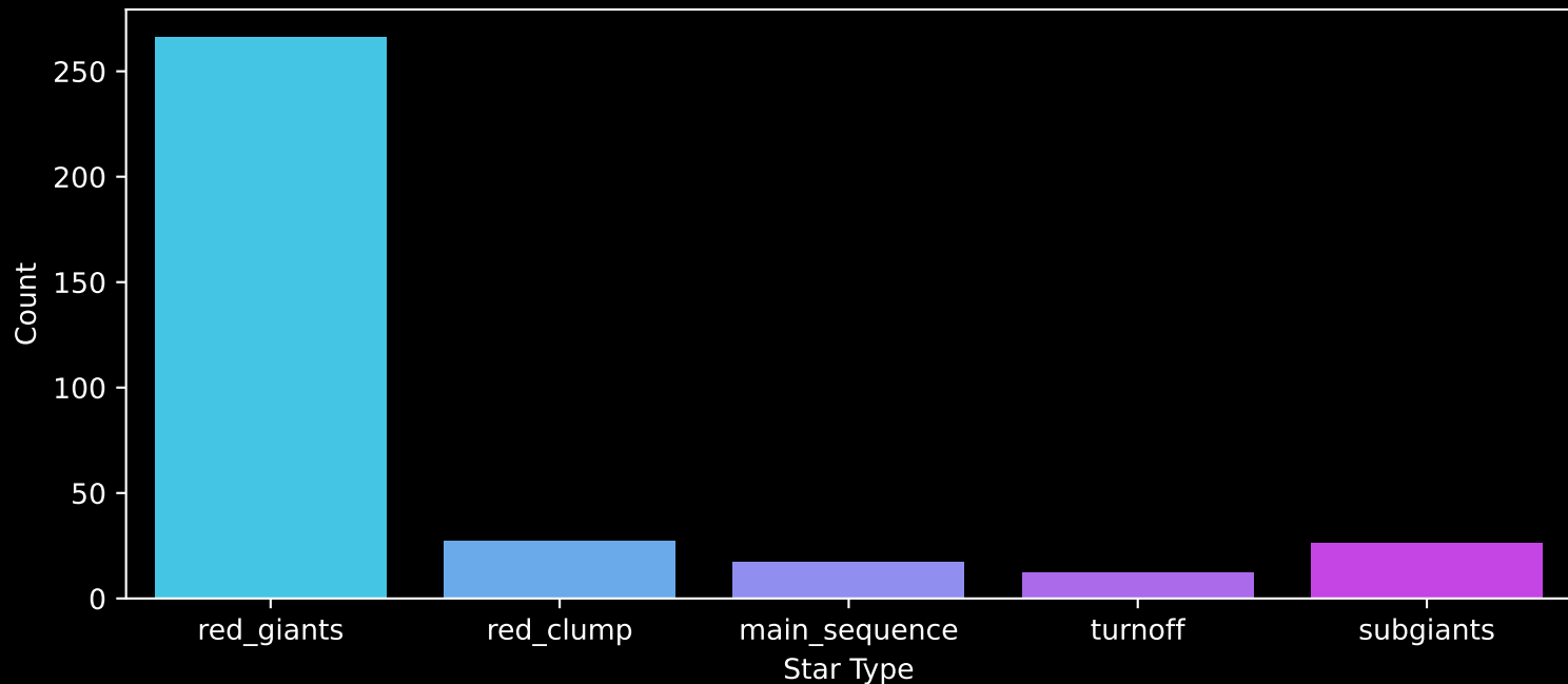
APOGEE DR17 Field: [188+00] Count plot of Star Type
